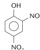
2,4-dinitrofenol
