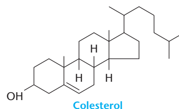
Colesterol
