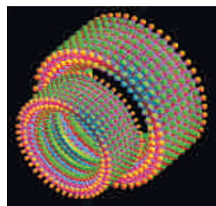
Nanotubo
